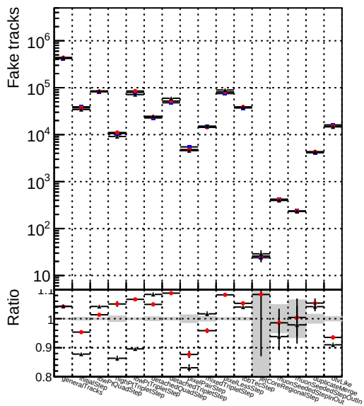
Number of tracks vs collection Legend: DQM_CKF_TTbase DQM_CKF_TT_retrainOldFiles113 DQM_CKF_TT_retrainOldFiles125
