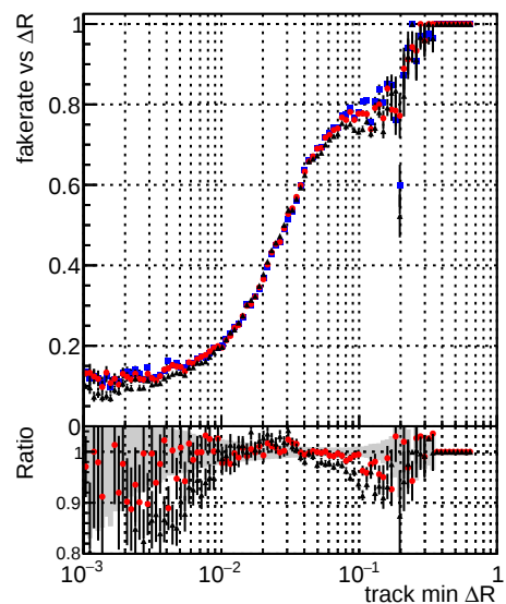
Fake rate vs \Delta R (track, jet) Legend: DOM_CKF_TTbase (black circles) DOM_CKF_TT_retrainOldFiles113 (red circles) DOM_CKF_TT_retrainOldFiles125 (blue circles)
