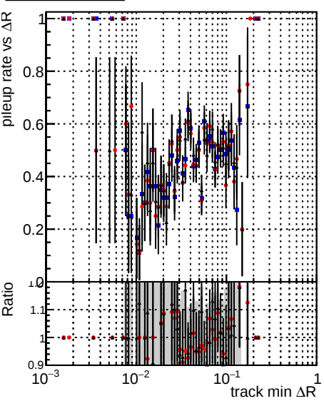
Legend: DQM_CKF_TTbase (black), DQM_CKF_TT_retrainOldFiles113 (red), DQM_CKF_TT_retrainOldFiles125 (blue)
