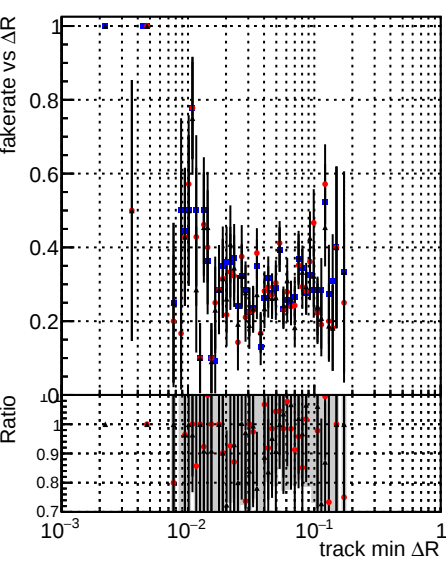
Legend: DQM_CKF_TTbase (black), DQM_CKF_TT_retrainOldFiles113 (red), DQM_CKF_TT_retrainOldFiles125 (blue)
