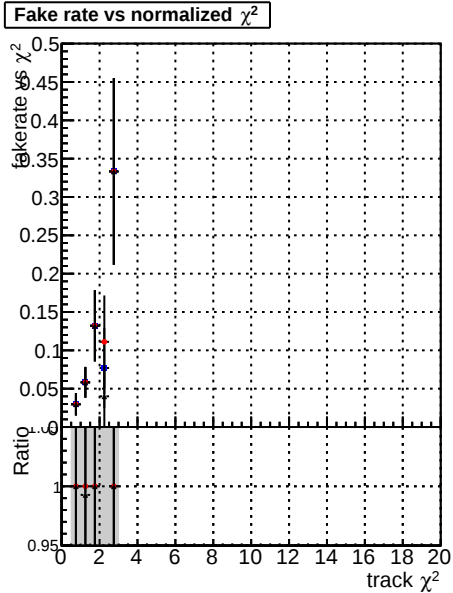
Fake rate vs. Legend: DOM (black), CKF (red), TTbase (blue), retrainOldFiles113 (green)
