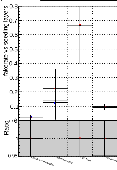
Fake rate vs. Legend: DOM (black), CKF (red), TTbase (blue), retrainOldFiles113 (green)
