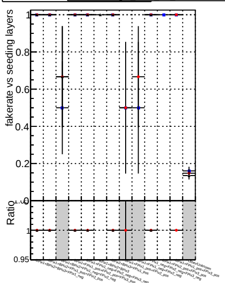
Fake rate vs. DOM CKF TTbase DOM CKF retrainOldFiles113 DOM CKF retrainOldFiles125
