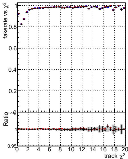
Fake rate vs. —■— DGM —●— CKF —▲— TTbase —×— retrainOldFiles113
