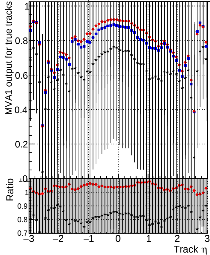
MVA1 of associated tracks (recoToSim) vs. track \eta Legend: DQM_CKF_TTbase (blue squares) DQM_CKF_TT_retrainOldFiles113 (red circles) DQM_CKF_TT_retrainOldFiles125 (black triangles)
