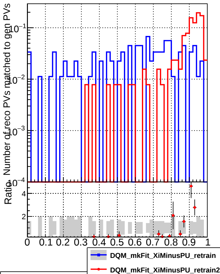
RecoPVAssoc2GenPVmatched_missing
