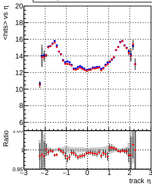
mean hits vs \eta Legend: DQM_mkFit_XiMinusPU_retrain (blue line), DQM_mkFit_XiMinusPU_retrain2 (red line)
