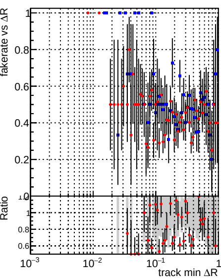
Legend: DQM_mkFit_XiMinusPU_retrain (blue dots), DQM_mkFit_XiMinusPU_retrain2 (red dots)
