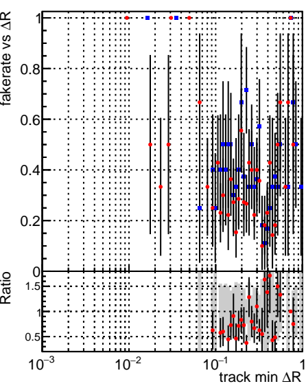
Fake rate vs \Delta R(\text{track, jet}) Legend: - Blue square: DQM_mkFit_XiMinusPU_retrain - Red circle: DQM_mkFit_XiMinusPU_retrain2
