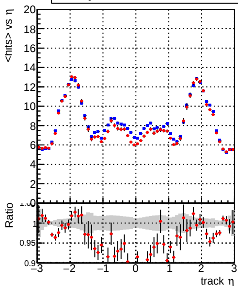
mean hit — DQM_mkJit_XiMinusPU_retrain — DQM_mkJit_XiMinusPU_retrain2
