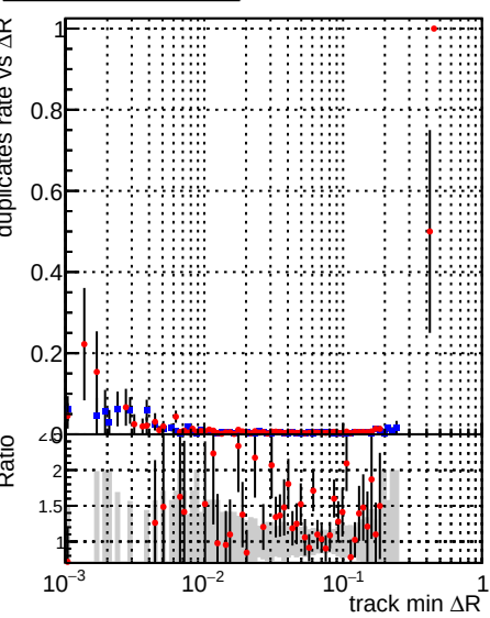
Legend: DQM_mkFit_XiMinusPU_retrain (blue), DQM_mkFit_XiMinusPU_retrain2 (red)
