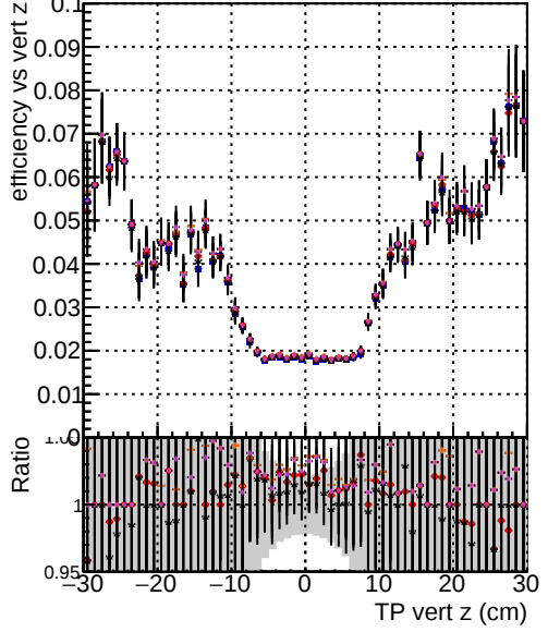
Efficiency vs vertpos DOM mkFit XiMinusNOPU new-lowpt DOM mkFit XiMinusNOPU NEWdefault specPLess1 DOM mkFit XiMinusNOPU NEWdefault specPLess2 DOM mkFit XiMinusNOPU NEWdefault specPLess3 DOM mkFit XiMinusNOPU NEWdefault specPLess4
