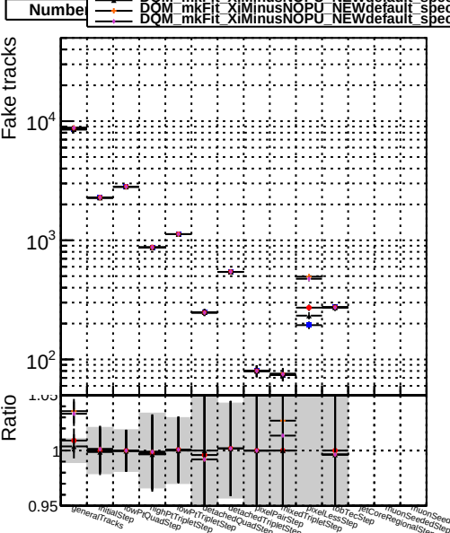
DOM mkFit6 XiMinusNOPU new-lowpt DOM mkFit6 XiMinusNOPU NEWdefau
