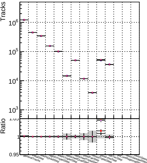
DOM mkFit6 XiMinusNOPU new-lowpt DOM mkFit6 XiMinusNOPU NEWdefau
