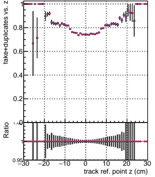
Legend for Efficiency vs. vert z: DQM mkFit XiMinusNOPU new_lowpt Legend for fake+duplicates vs. vert z: DQM mkFit XiMinusNOPU NEWdefault specPLess1 Legend for Efficiency vs. sim PV z: DQM mkFit XiMinusNOPU NEWdefault specPLess3 Legend for fake+duplicates vs. sim PV z: DQM mkFit XiMinusNOPU NEWdefault specPLess4
