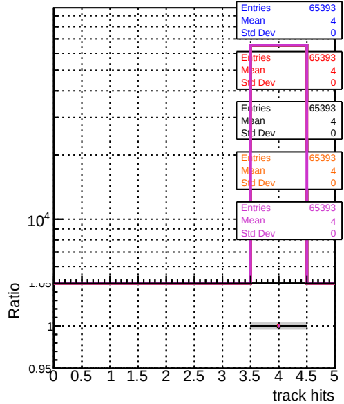
track hits
