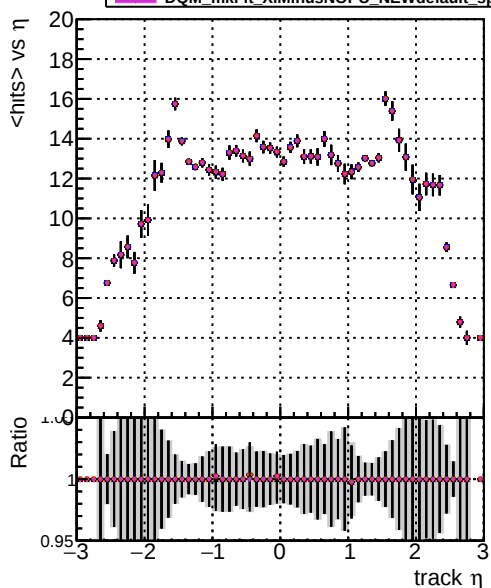
mean hit DOM mkFit XiMinusNOPU NEWdefault specPless1 DOM mkFit XiMinusNOPU NEWdefault specPless2 DOM mkFit XiMinusNOPU NEWdefault specPless3 DOM mkFit XiMinusNOPU NEWdefault specPless4
