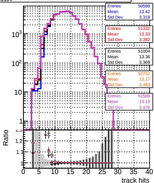
Legend: DOM mkFit XiMinusNOPU NEWdefault specPless1, DOM mkFit XiMinusNOPU NEWdefault specPless2, DOM mkFit XiMinusNOPU NEWdefault specPless3, DOM mkFit XiMinusNOPU NEWdefault specPless4 mean hits
