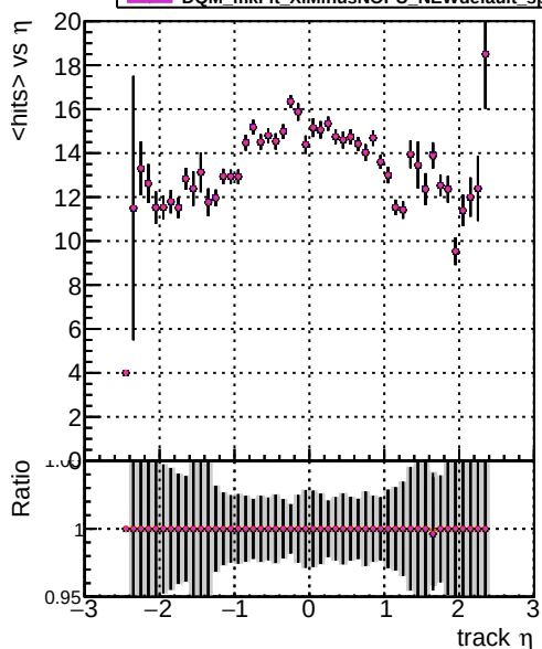
Legend: DOM mkFit XiMinusNOPU NEWlowpt specPless1 DOM mkFit XiMinusNOPU NEWdefault specPless2 DOM mkFit XiMinusNOPU NEWdefault specPless3 DOM mkFit XiMinusNOPU NEWdefault specPless4 mean hit
