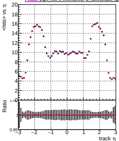
Legend for mean hits vs \eta : DOM mkFit XiMinusNOPU NEWdefault specPless1 DOM mkFit XiMinusNOPU NEWdefault specPless2 DOM mkFit XiMinusNOPU NEWdefault specPless3 DOM mkFit XiMinusNOPU NEWdefault specPless4
