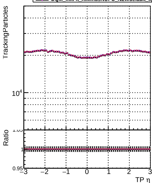
N of sim Model Method Model Method Model Method Model Method 100 DOM mkFit XiMinus NOPU NEWdefault specPless2 100 DOM mkFit XiMinus NOPU NEWdefault specPless3 100 DOM mkFit XiMinus NOPU NEWdefault specPless3
