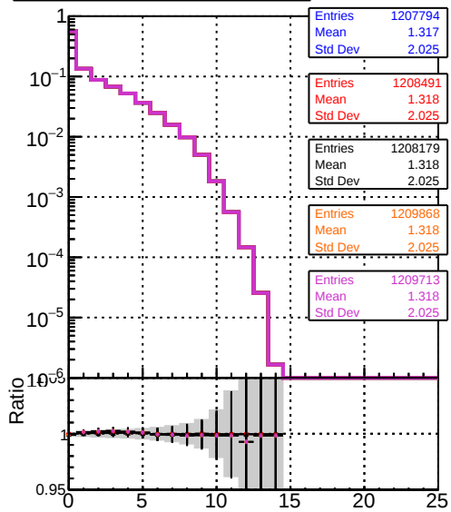
mean hit DOM mkFit XiMinusNOPU new_lowpt specPless1 DOM mkFit XiMinusNOPU NEWdefault specPless2 DOM mkFit XiMinusNOPU NEWdefault specPless3 DOM mkFit XiMinusNOPU NEWdefault specPless4
