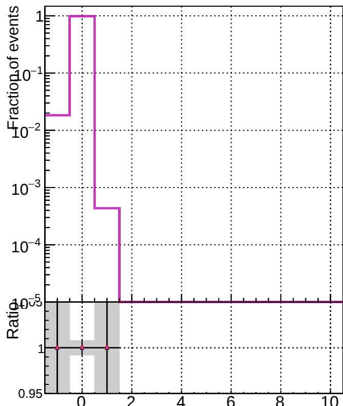
Index of signal PV in reco collection
