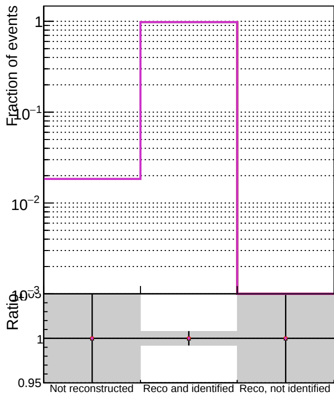
Signal PV status in reco collection
