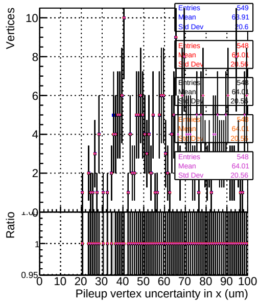
Legend: DOM mkFit XiMinusNOPU NEWdefault specLess1, DOM mkFit XiMinusNOPU NEWdefault specLess3, DOM mkFit XiMinusNOPU NEWdefault specLess4
