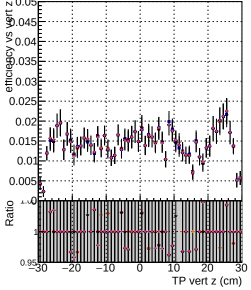
Efficiency vs. sim PV z DOM mkFit XiMinusNOPU NEWdefault specLess1 DOM mkFit XiMinusNOPU NEWdefault specLess2 DOM mkFit XiMinusNOPU NEWdefault specLess3 DOM mkFit XiMinusNOPU NEWdefault specLess4
