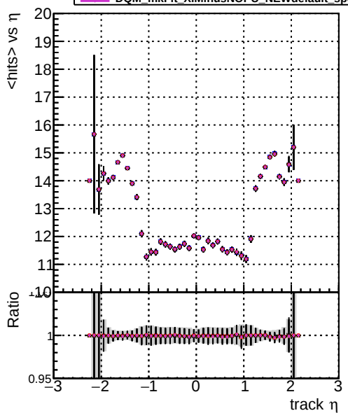
mean hits DOM mkFit XiMinusNOPU NEWdefault specPless1 DOM mkFit XiMinusNOPU NEWdefault specPless2 DOM mkFit XiMinusNOPU NEWdefault specPless3 DOM mkFit XiMinusNOPU NEWdefault specPless4
