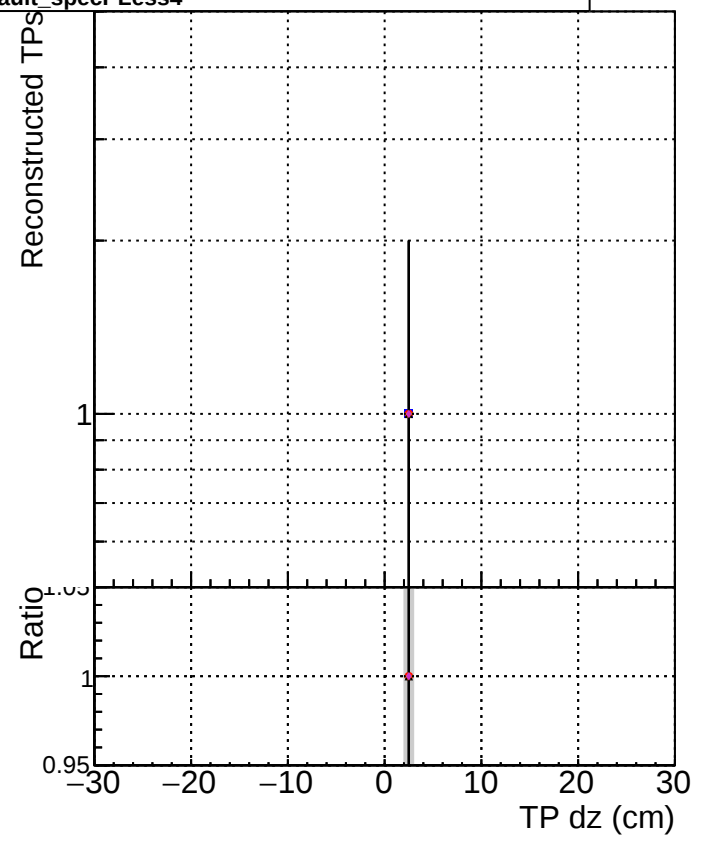
N of simulated track DOM_mkFit6_XiMinusNOPUnew-lowpt DOM_mkFit6_XiMinusNOPU_NEWdefault_specPless1 DOM_mkFit6_XiMinusNOPU_NEWdefault_specPless2 DOM_mkFit6_XiMinusNOPU_NEWdefault_specPless3 DOM_mkFit6_XiMinusNOPU_NEWdefault_specPless4
