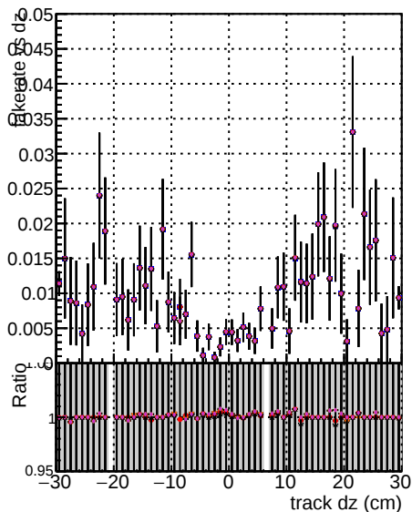
DOM mkt F6 X Y Minus NOP New Low Up Fake rate vs d
