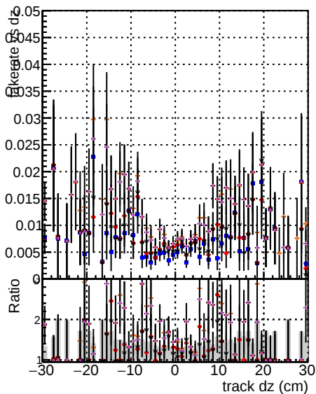
Fake rate vs d DOM m k Fit i6 Xi Minus NOPU new low p t
