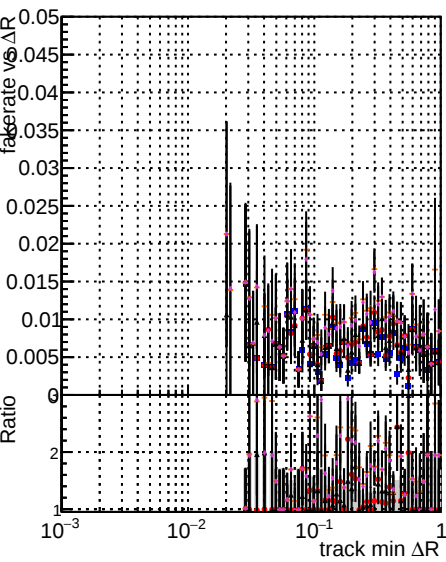
Fake rate vs \Delta R(\text{track, jet}) Legend: DOM (black), mkFit6 (blue), XiMinus (red), NOPU (green), NewLowpt (purple), NewDefault (orange), specBLess1 (grey), specBLess2 (light grey), specBLess3 (dark grey), specBLess4 (very dark grey).
