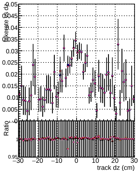
Fake rate vs d DOM mkt Fit 6 Xi Minus NOPU New low pT W Z B L S D C P E S S 1 2 3 4
