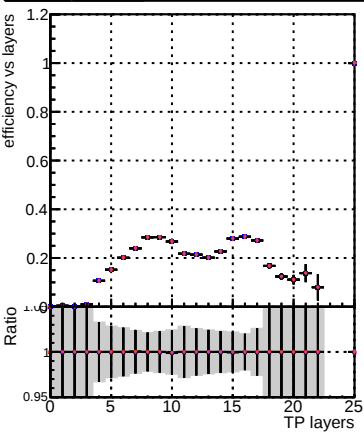
Efficiency vs hit Legend: DOM_mkFit6_TTnew-lowpt DOM_mkFit_TT_NEWdefault_specPless1-lowpt DOM_mkFit_TT_NEWdefault_specPless2-lowpt DOM_mkFit_TT_NEWdefault_specPless3-lowpt DOM_mkFit_TT_NEWdefault_specPless4-lowpt
