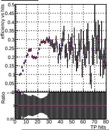
Efficiency vs hit Legend: DOM_mkFit6_TTnew-lowpt DOM_mkFit_TT_NEWdefault_specPless1-lowpt DOM_mkFit_TT_NEWdefault_specPless2-lowpt DOM_mkFit_TT_NEWdefault_specPless3-lowpt DOM_mkFit_TT_NEWdefault_specPless4-lowpt
