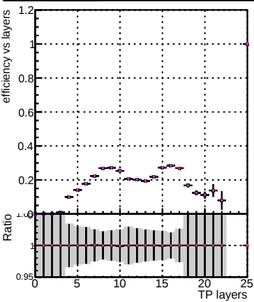
Efficiency vs hit DOM_mkFit6_TTnew_lowpt DOM_mkFit_TT_NEWdefault_specPless1_lowpt DOM_mkFit_TT_NEWdefault_specPless2_lowpt DOM_mkFit_TT_NEWdefault_specPless3_lowpt DOM_mkFit_TT_NEWdefault_specPless4_lowpt
