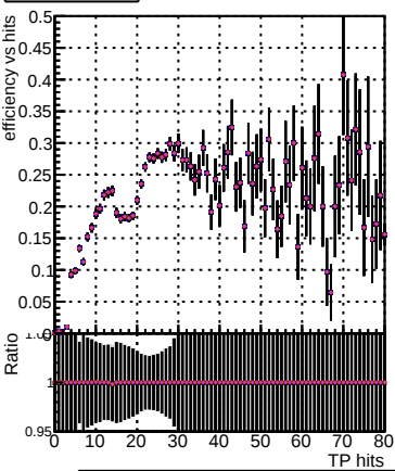
Efficiency vs hit DOM_mkFit6_TTnew_lowpt DOM_mkFit_TT_NEWdefault_specPless1_lowpt DOM_mkFit_TT_NEWdefault_specPless2_lowpt DOM_mkFit_TT_NEWdefault_specPless3_lowpt DOM_mkFit_TT_NEWdefault_specPless4_lowpt
