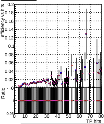
Efficiency vs hit DOM_mkFit_tt1new-lowpt DOM_mkFit_tt_NEWdefault_specPless1-lowpt DOM_mkFit_tt_NEWdefault_specPless2-lowpt DOM_mkFit_tt_NEWdefault_specPless3-lowpt DOM_mkFit_tt_NEWdefault_specPless4-lowpt
