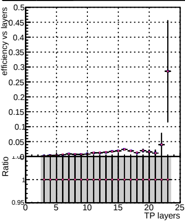
Efficiency vs hit DOM_mkFit_tt1new-lowpt DOM_mkFit_tt_NEWdefault_specPless1-lowpt DOM_mkFit_tt_NEWdefault_specPless2-lowpt DOM_mkFit_tt_NEWdefault_specPless3-lowpt DOM_mkFit_tt_NEWdefault_specPless4-lowpt
