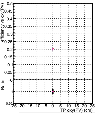
Efficiency vs Dxy(PV) legend DQM_mkFit6_11new-lowpt DQM_mkFit_TT_NEWdefault_specPless1-lowpt DQM_mkFit_TT_NEWdefault_specPless2-lowpt DQM_mkFit_TT_NEWdefault_specPless3-lowpt DQM_mkFit_TT_NEWdefault_specPless4-lowpt
