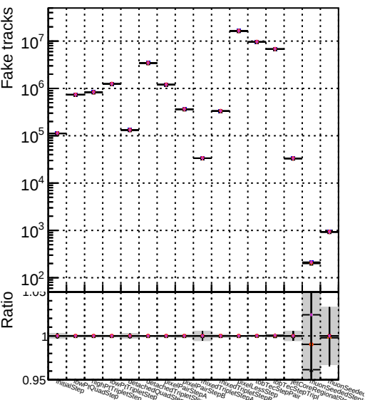
Number Symbol DOM mkFit TT NEWdefault specP Less2 lowpt DOM mkFit TT NEWdefault specP Less2 lowpt DOM mkFit TT NEWdefault specP Less3 lowpt DOM mkFit TT NEWdefault specP Less4 lowpt
