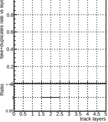
fake+duplicates vs layers
