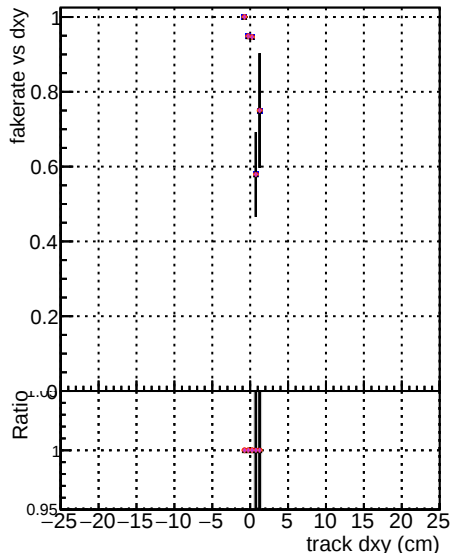
DOM mkFit TT new lowpt DOM mkFit TT new lowpt DOM mkFit TT new lowpt
