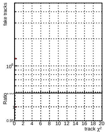
N of associated (recoToSim) fake tracks vs. \chi^2 bins
