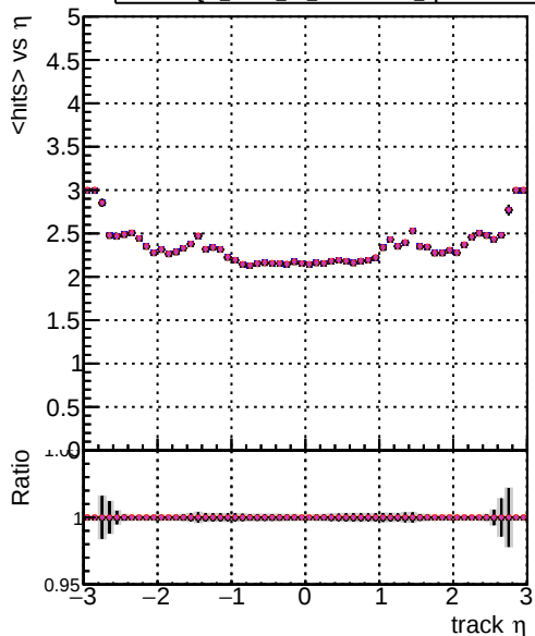
Legend for mean hits vs track \eta : DOM mkFit TT NEWdefault specPless1-lowpt DOM mkFit TT NEWdefault specPless2-lowpt DOM mkFit TT NEWdefault specPless3-lowpt DOM mkFit TT NEWdefault specPless4-lowpt
