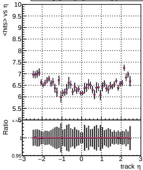
Legend: DOM mkFit TT NEWdefault specPLess1-lowpt, DOM mkFit TT NEWdefault specPLess2-lowpt, DOM mkFit TT NEWdefault specPLess3-lowpt, DOM mkFit TT NEWdefault specPLess4-lowpt mean hits
