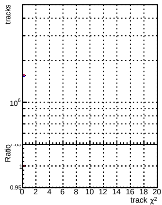
N of reco track vs. \chi^2 (new lower)
