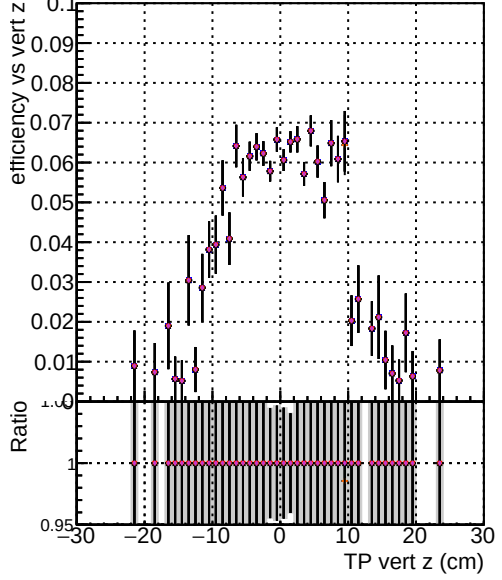
Efficiency vs. TP vert z (cm) DOM mkFit TT NEWdefault specPLess1-lowpt DOM mkFit TT NEWdefault specPLess2-lowpt DOM mkFit TT NEWdefault specPLess3-lowpt DOM mkFit TT NEWdefault specPLess4-lowpt
