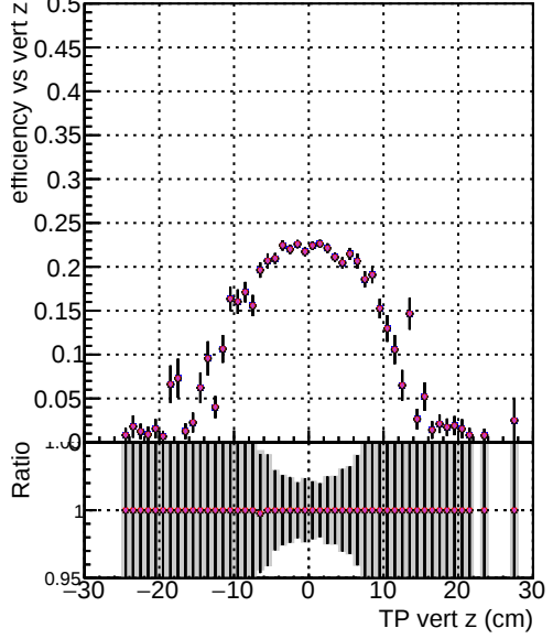
Efficiency vs. TP vert z — DOM mkFit TT NEWdefault specPless1-lowpt — DOM mkFit TT NEWdefault specPless2-lowpt — DOM mkFit TT NEWdefault specPless3-lowpt — DOM mkFit TT NEWdefault specPless4-lowpt
