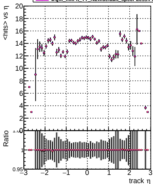
Legend: DOM mkFit TT NEWdefault specPless1-lowpt, DOM mkFit TT NEWdefault specPless2-lowpt, DOM mkFit TT NEWdefault specPless3-lowpt, DOM mkFit TT NEWdefault specPless4-lowpt mean hits vs \eta
