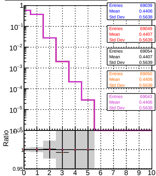
Legend for mean hits vs \eta : DOM mkFit TT NEWdefault specPless1-lowpt DOM mkFit TT NEWdefault specPless2-lowpt DOM mkFit TT NEWdefault specPless3-lowpt DOM mkFit TT NEWdefault specPless4-lowpt
