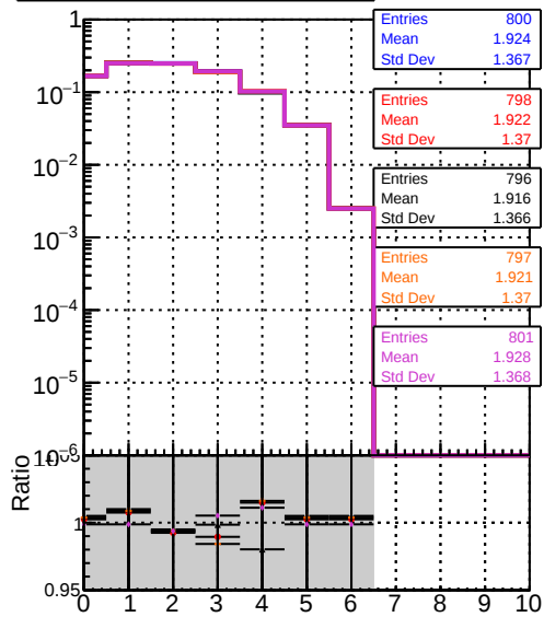
mean hit Legend: DOM mkFit TT NEWdefault specPless1-lowpt DOM mkFit TT NEWdefault specPless2-lowpt DOM mkFit TT NEWdefault specPless3-lowpt DOM mkFit TT NEWdefault specPless4-lowpt
