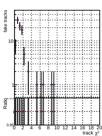
N of fake tracks vs. s
