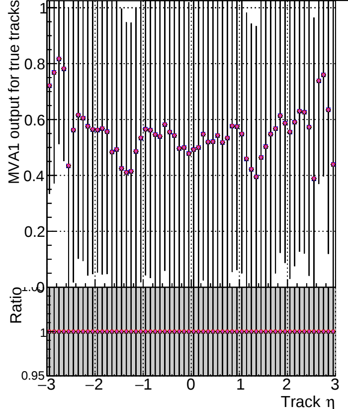
MVA1 of associated tracks (recoToSim) vs. track \eta Legend: DOM mkFit6 TTnew-lowpt DOM mkFit TT NEWdefault specPless1-lowpt DOM mkFit TT NEWdefault specPless2-lowpt DOM mkFit TT NEWdefault specPless3-lowpt DOM mkFit TT NEWdefault specPless4-lowpt
